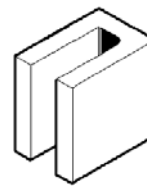
15-93 190 x 190 x 140 Half stop-end 4.5kg 252 per pallet
