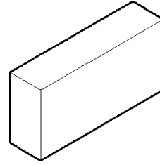
10-31 390 x 190 x 90 Full solid 10.8kg 144 per pallet
