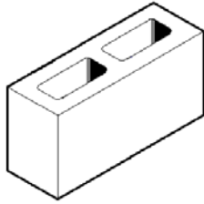
15-01 390 x 190 x 140 Full block 9.4kg 144 per pallet
