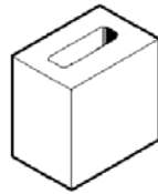
15-403 190 x 190 x 140 4-hour half block 7.6kg 252 per pallet
