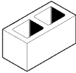
20-01 390 x 190 x 190 Full block 12.0kg 108 per pallet
