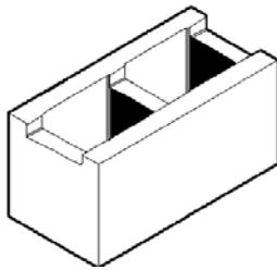
20-42 390 x 190 x 190 Recessed web 11.5kg 108 per pallet
