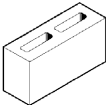
15-401 390 x 190 x 140 4-hour full block 14.8kg 120 per pallet
