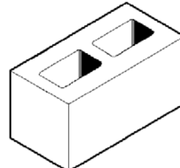
20-401 390 x 190 x 190 4-hour full block 16.0kg 90 per pallet
