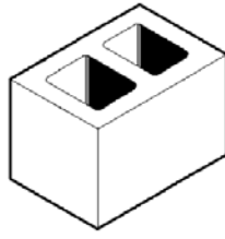
20-02 290 x 190 x 190 3/4 block 9.2kg 120 per pallet
