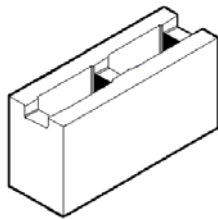
15-42 390 x 190 x 140 Recessed webs 9.7kg 144 per pallet
