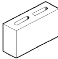
10-02 290 x 190 x 90 Three-quarter 7.0kg 240 per pallet
