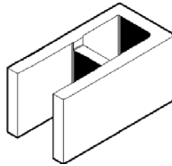
20-92 390 x 190 x 190 Full stop-end 11.0kg 108 per pallet
