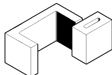
20-96 390 x 190 x 190 + 190 x 190 x 90 300mm Clean-out composite block 9.5kg + 4.0kg 90 per pallet
