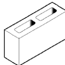
12-01 390 x 190 x 110 Hollow Brick-block 8.8kg 180 per pallet
