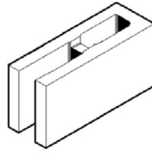
15-92 390 x 190 x 140 Full stop-end 9.0kg 144 per pallet
