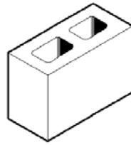
15-02 290 x 190 x 140 ¾ block 8.8kg 180 per pallet
