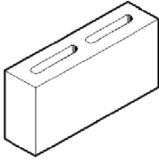
10-01 390 x 190 x 90 Full block 8.2kg 180 per pallet
