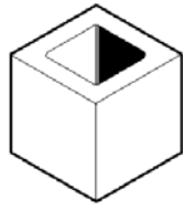
20-03 190 x 190 x 190 Half block 6.3kg 180 per pallet
