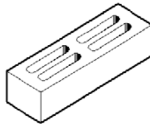
12-71C 390 x 90 x 110 Chaser Half-high 4.5kg 300 per pallet
