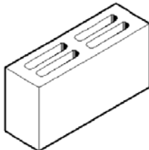
12-01C 390 x 190 x 110 Chaser Full 9.1kg 180 per pallet
