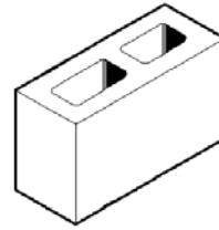
15-22 340 x 190 x 140 Corner block (7/8) 9.1kg 135 per pallet
