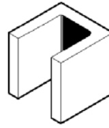
20-93 190 x 190 x 190 Half stop-end 5.0kg 180 per pallet
