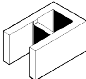
30-92 390 x 190 x 290 Full stop-end 16.5kg 72 per pallet
