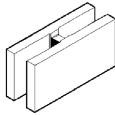
15-48 390 x 190 x 140 "H" block 10.0kg 120 per pallet
